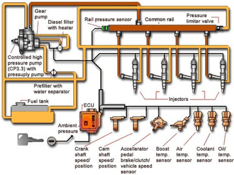
Common Rail System: Main components
